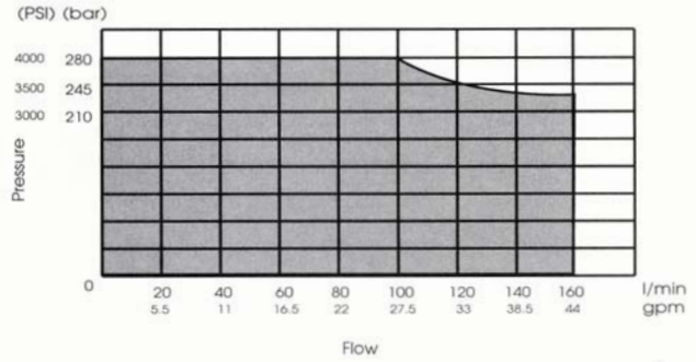
Pressure drop
